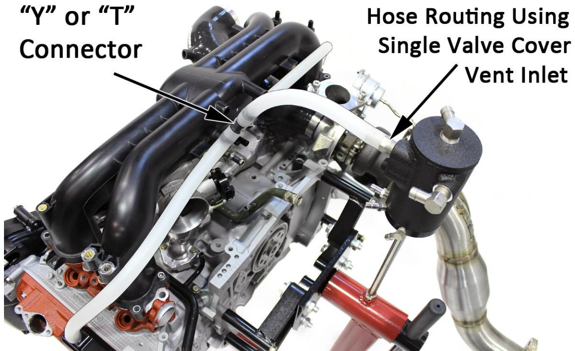
Diagram shows simplified hose routing for 08-14 WRX.
